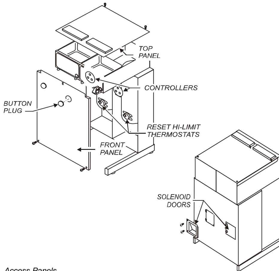
Fig. 12 Access Panels
